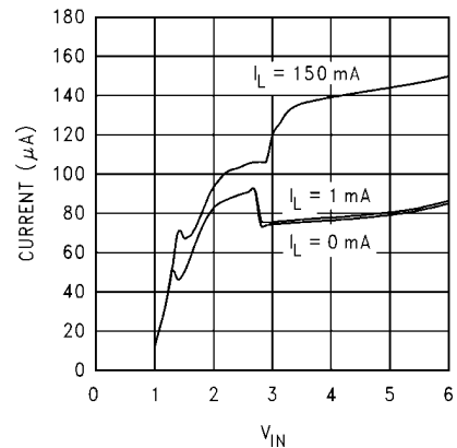
Ground Current vs V_{IN} @ 25°C
